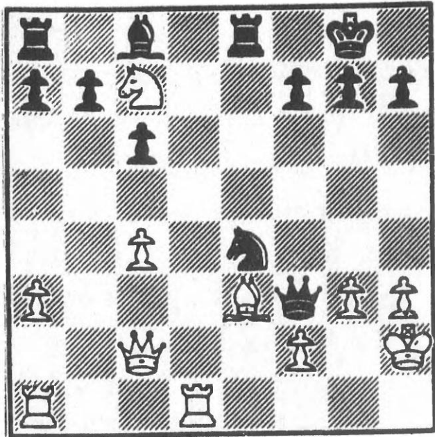
377 After 22 Kh2
